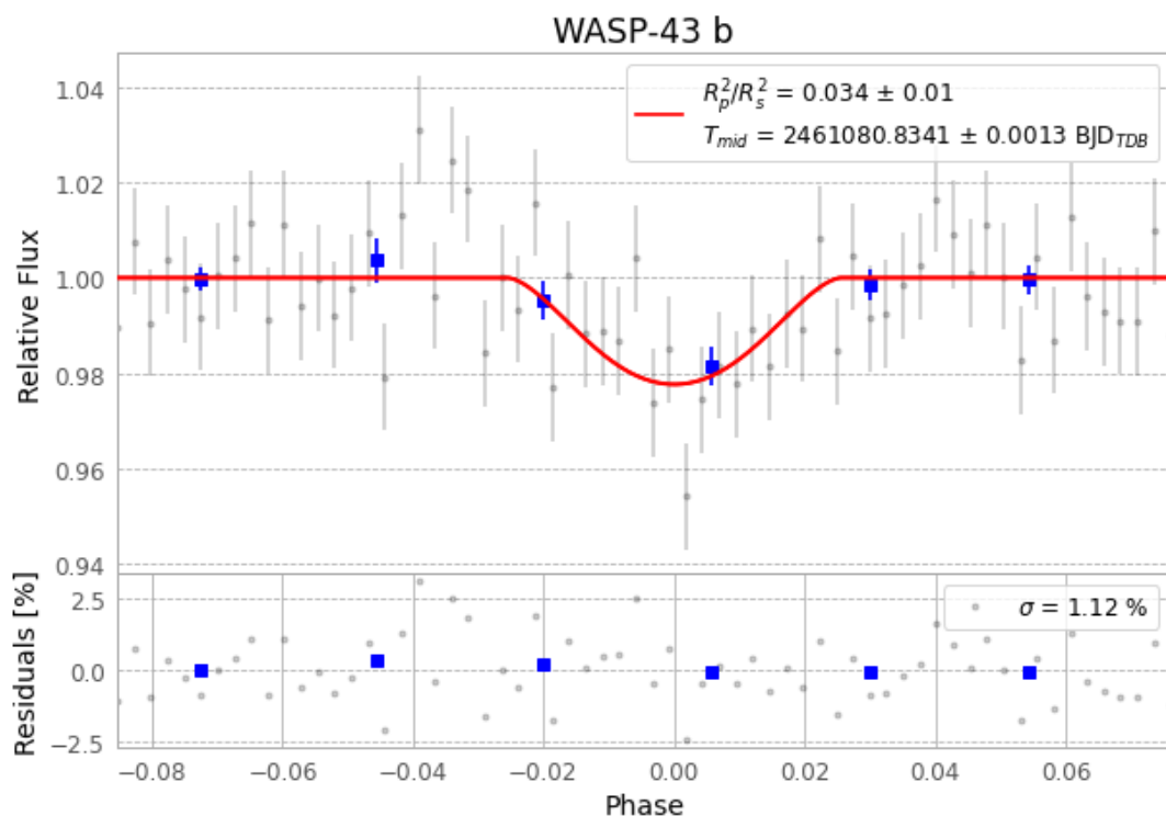
Figure 1 — FinalLightCurve_WASP-43 b_2026-02-08.png (SHA-256 00897090559dbaa2...)
