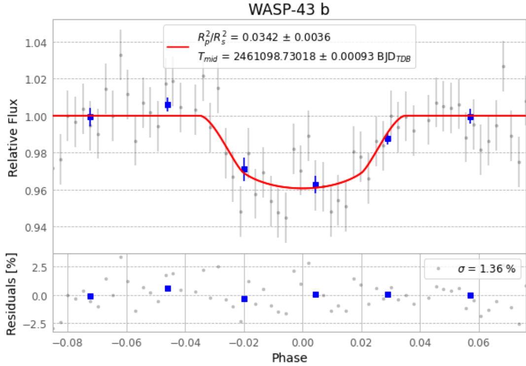
Figure 1 — FinalLightCurve_WASP-43 b_2026-02-26.png (SHA-256 fcb6d6f39829e9b...)
