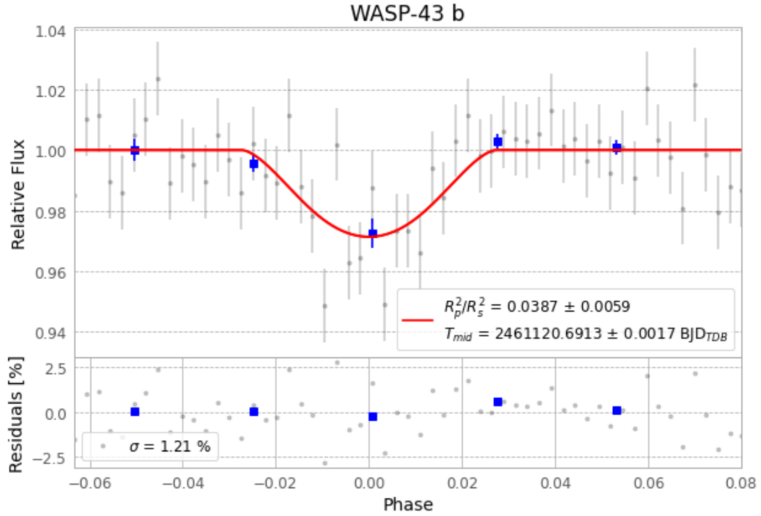
Figure 1 — FinalLightCurve_WASP-43 b_2026-03-20.png (SHA-256 4d2c074615dabd36...)
