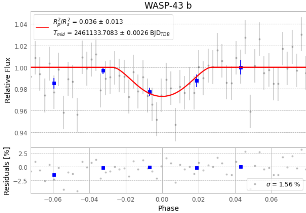
Figure 1 — FinalLightCurve_WASP-43 b_2026-04-02.png (SHA-256 304db135159cd9ee...)
