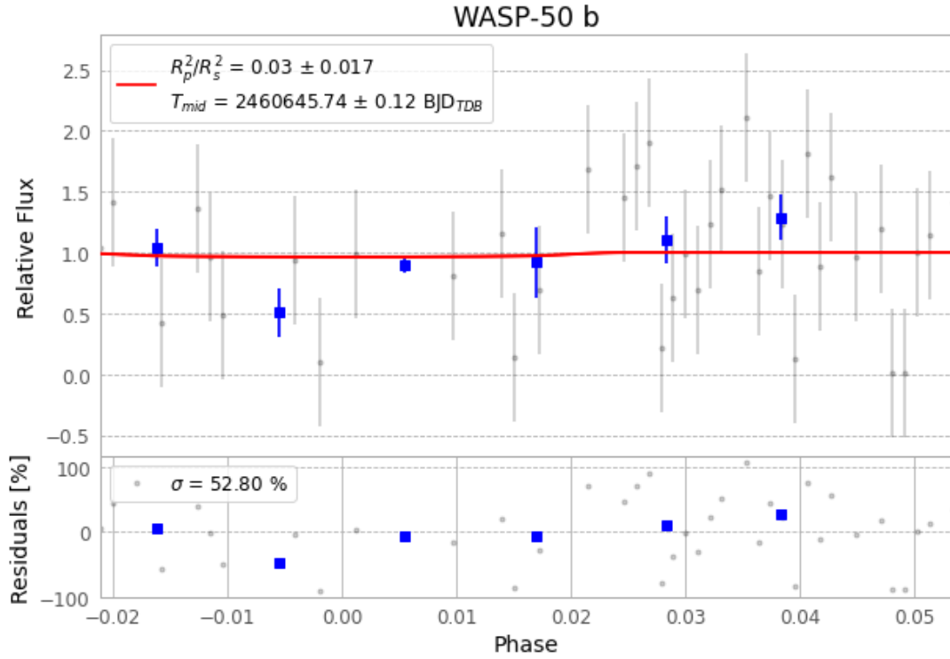
Figure 1 — FinalLightCurve_WASP-50 b_2024-11-30.png (SHA-256 c50af0ce8be893bc...)
