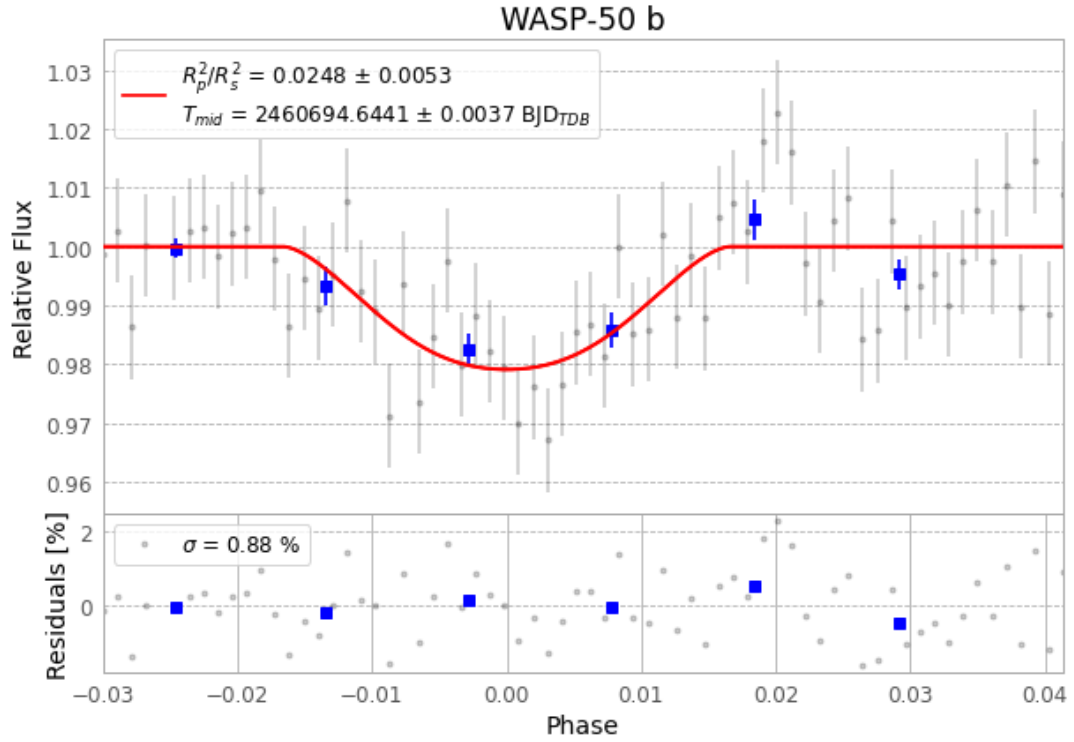
Figure 1 — FinalLightCurve_WASP-50 b_2025-01-18.png (SHA-256 2b0253a27fc9297e...)
