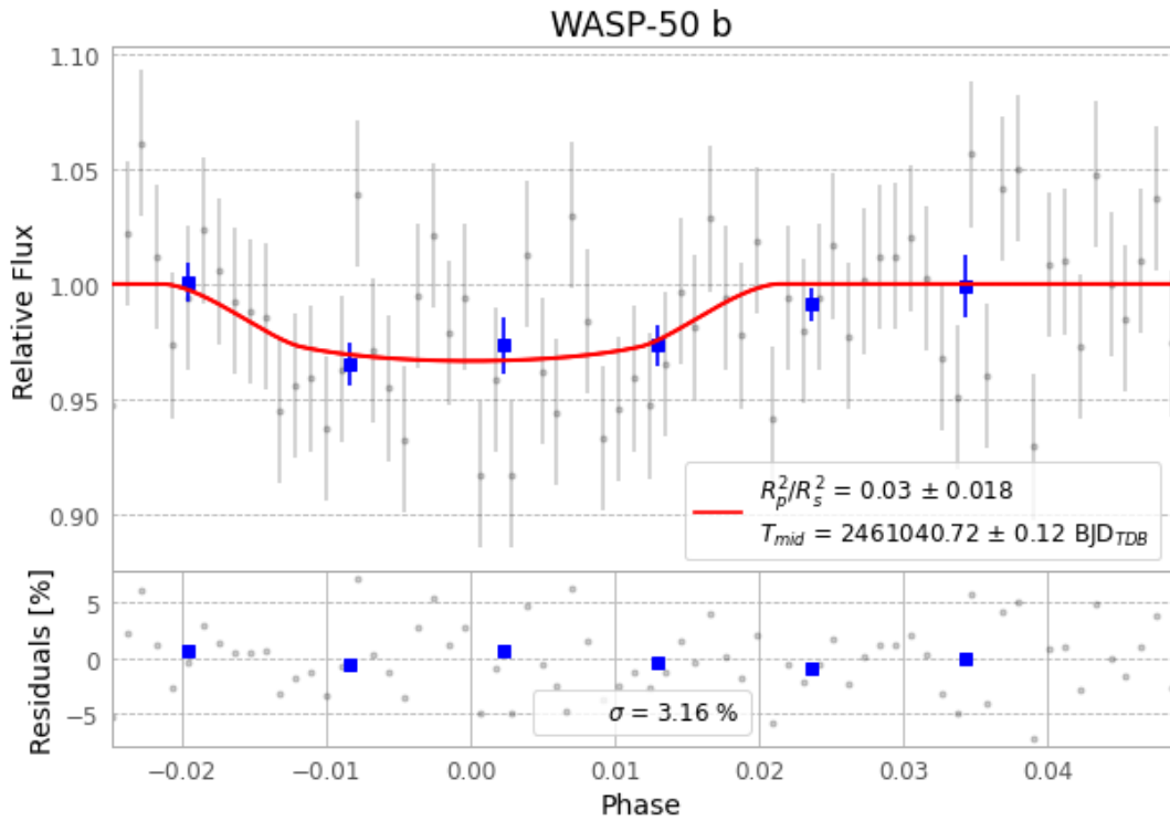
Figure 1 — FinalLightCurve_WASP-50 b_2025-12-30.png (SHA-256 50d82dcc63baec22...)
