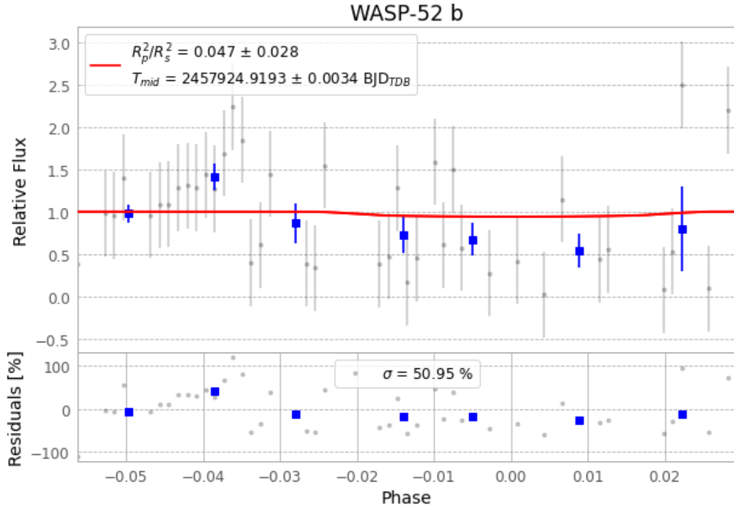
Figure 1 — FinalLightCurve_WASP-52 b_2017-06-20.png (SHA-256 94f3b642296e70aa...)
