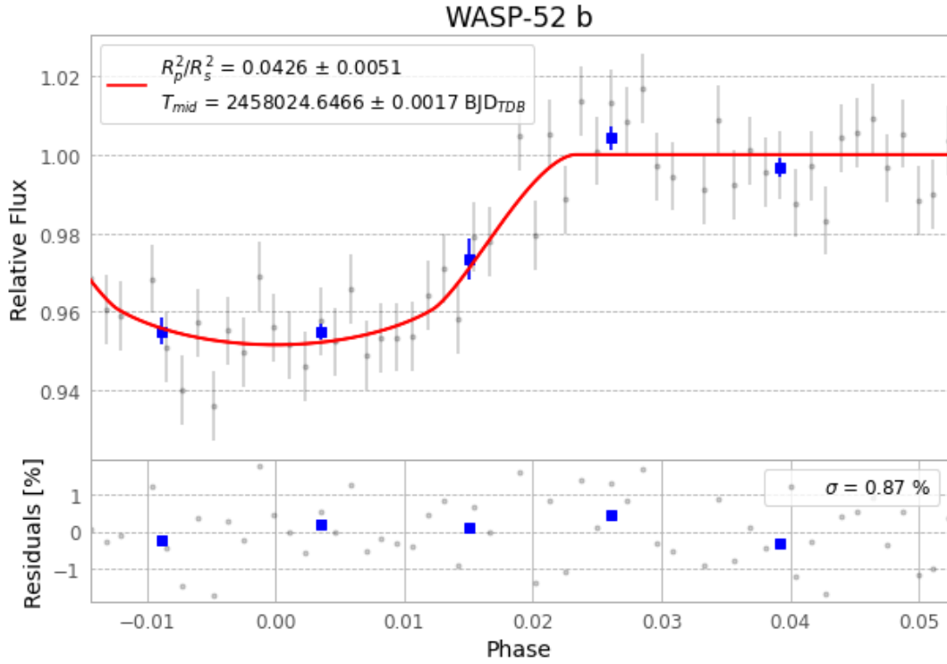
Figure 1 — FinalLightCurve_WASP-52 b_2017-09-27.png (SHA-256 e3d11b084c54a64a...)
