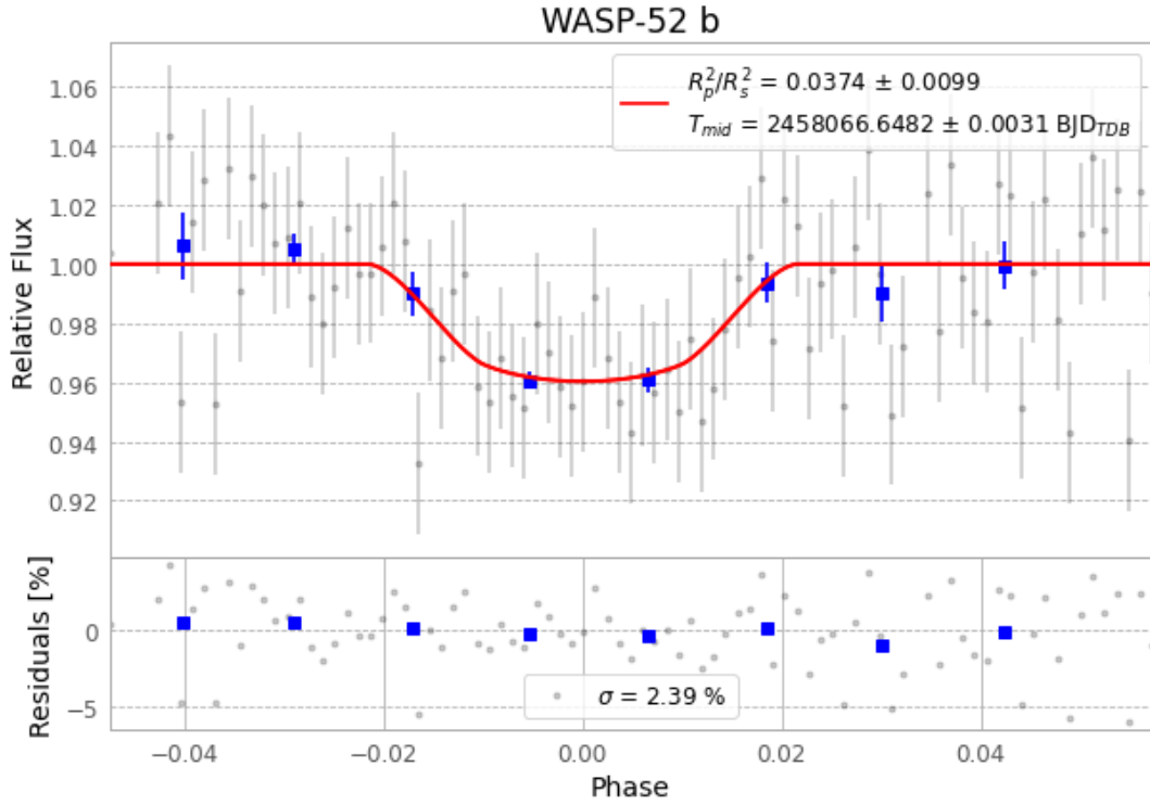
Figure 1 — FinalLightCurve_WASP-52 b_2017-11-08.png (SHA-256 6bba934ece02b5bd...)
