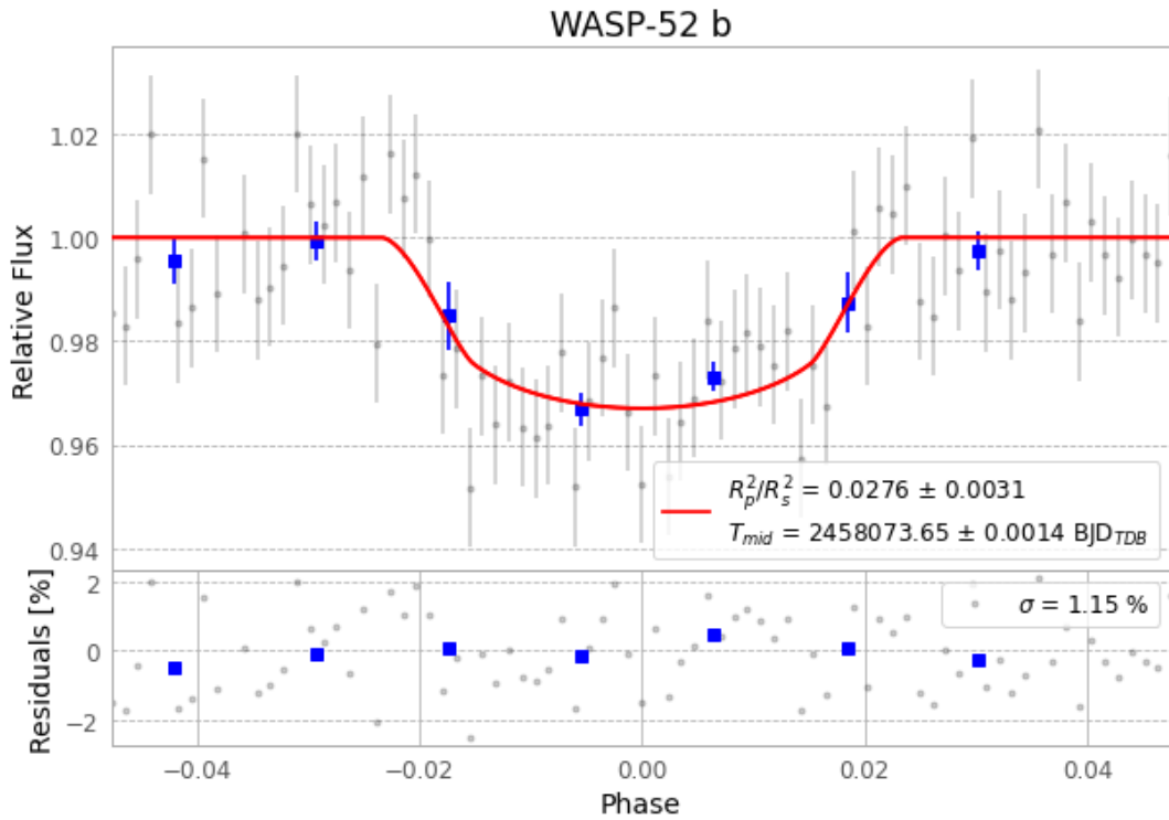
Figure 1 — FinalLightCurve_WASP-52 b_2017-11-15.png (SHA-256 931635d6fad4341d...)
