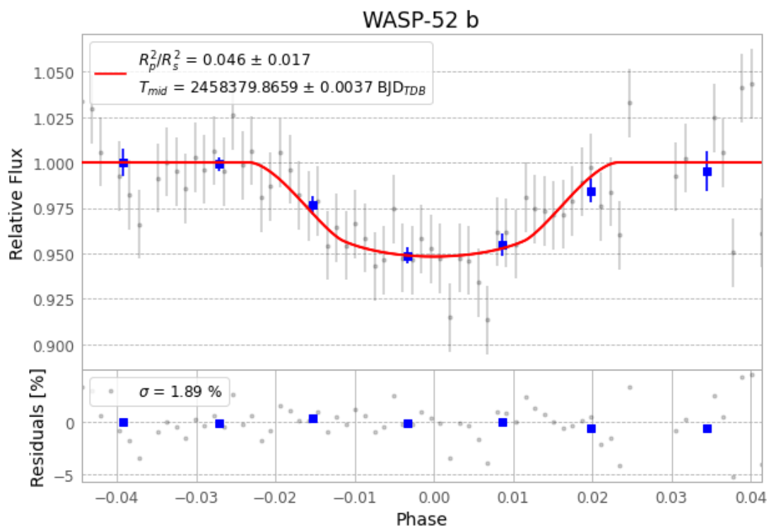
Figure 1 — FinalLightCurve_WASP-52 b_2018-09-17.png (SHA-256 46fcb2ada0fe74e2...)
