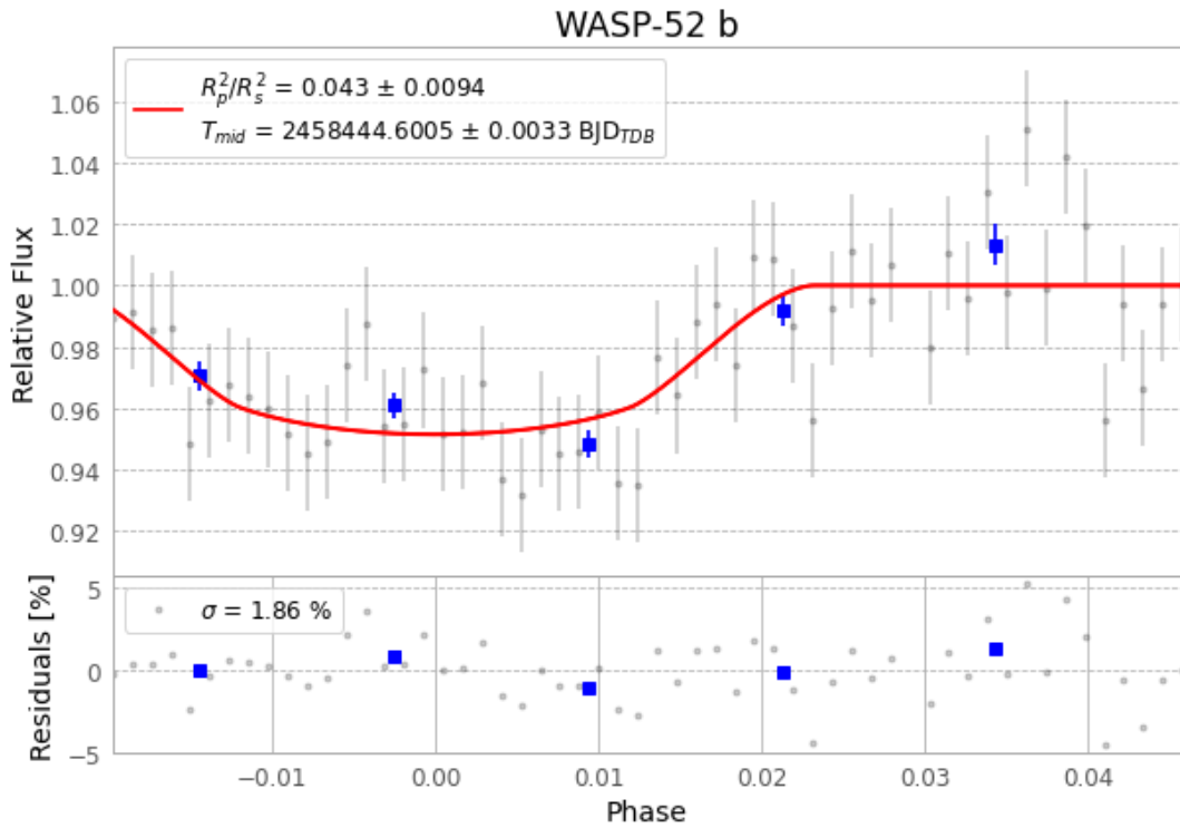
Figure 1 — FinalLightCurve_WASP-52 b_2018-11-21.png (SHA-256 6269ba877ffe12e7...)
