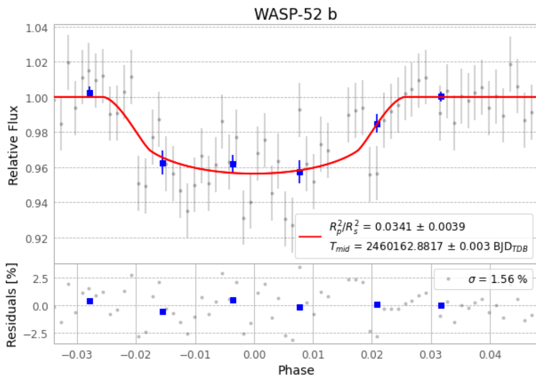
Figure 1 — FinalLightCurve_WASP-52 b_2023-08-06.png (SHA-256 88e762fe6658165e...)
