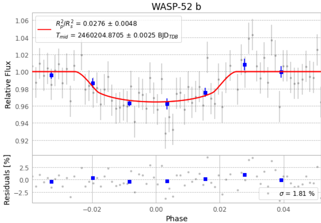
Figure 1 — FinalLightCurve_WASP-52 b_2023-09-17.png (SHA-256 f62a26cbce45f6b3...)
