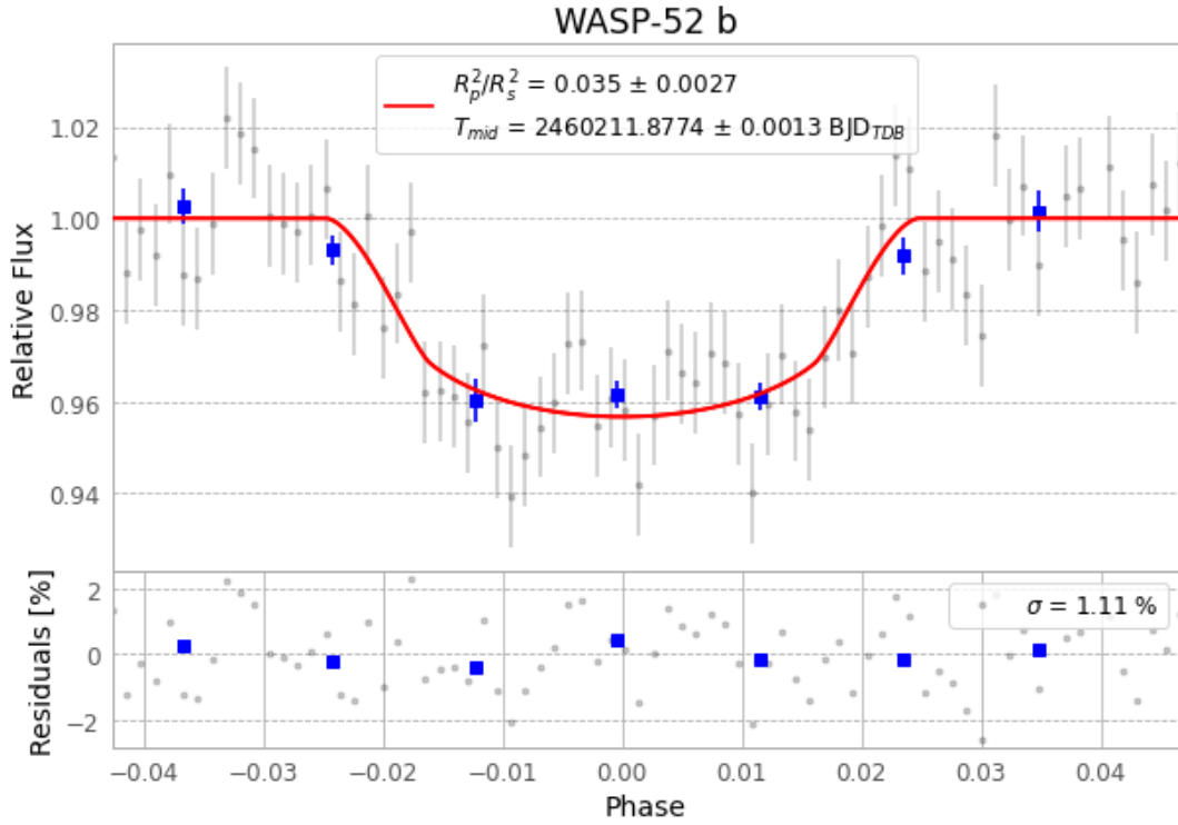
Figure 1 — FinalLightCurve_WASP-52 b_2023-09-24.png (SHA-256 064f90d7b5c9c78a...)
