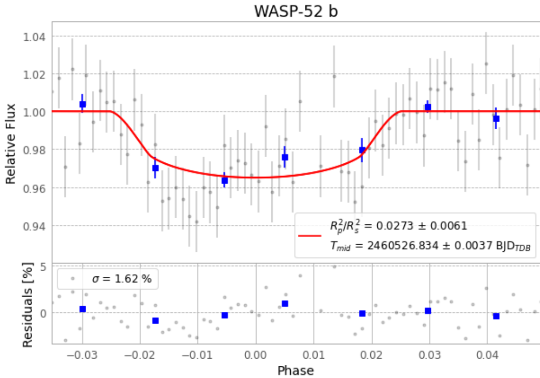
Figure 1 — FinalLightCurve_WASP-52 b_2024-08-03.png (SHA-256 1d88f5bf166d77b7...)
