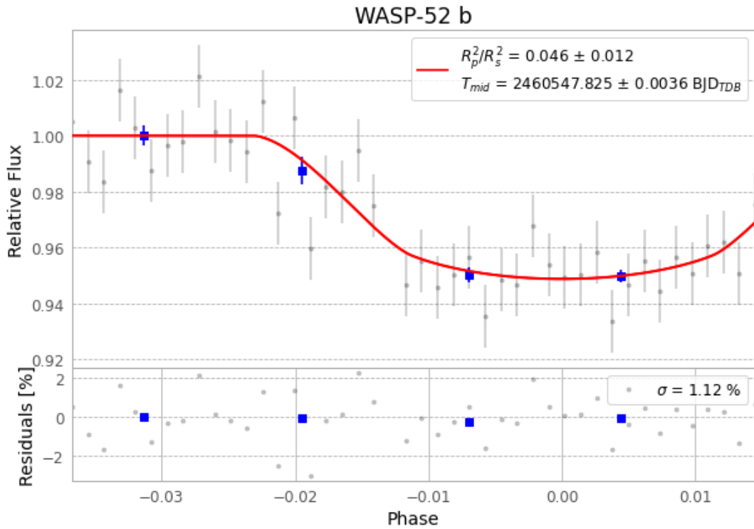
Figure 1 — FinalLightCurve_WASP-52 b_2024-08-24.png (SHA-256 3dc1f5f83a445032...)
