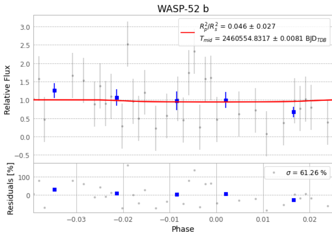
Figure 1 — FinalLightCurve_WASP-52 b_2024-08-31.png (SHA-256 fac4201113ea98fc...)
