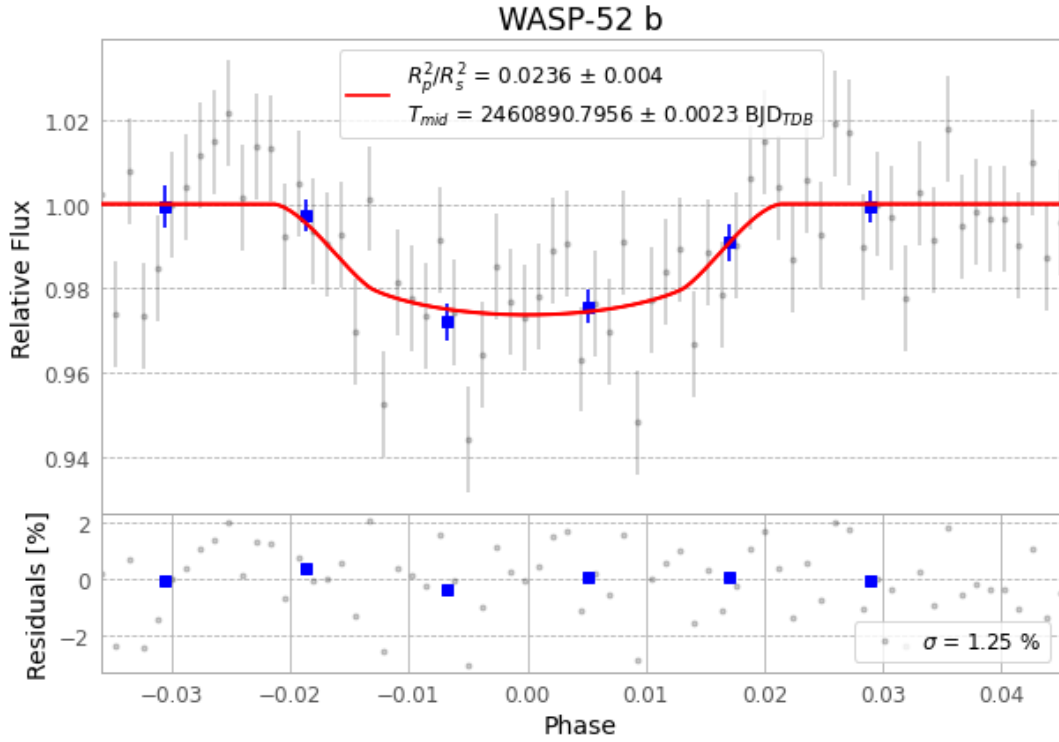
Figure 1 — FinalLightCurve_WASP-52 b_2025-08-02.png (SHA-256 3bf97152280f3ad9...)
