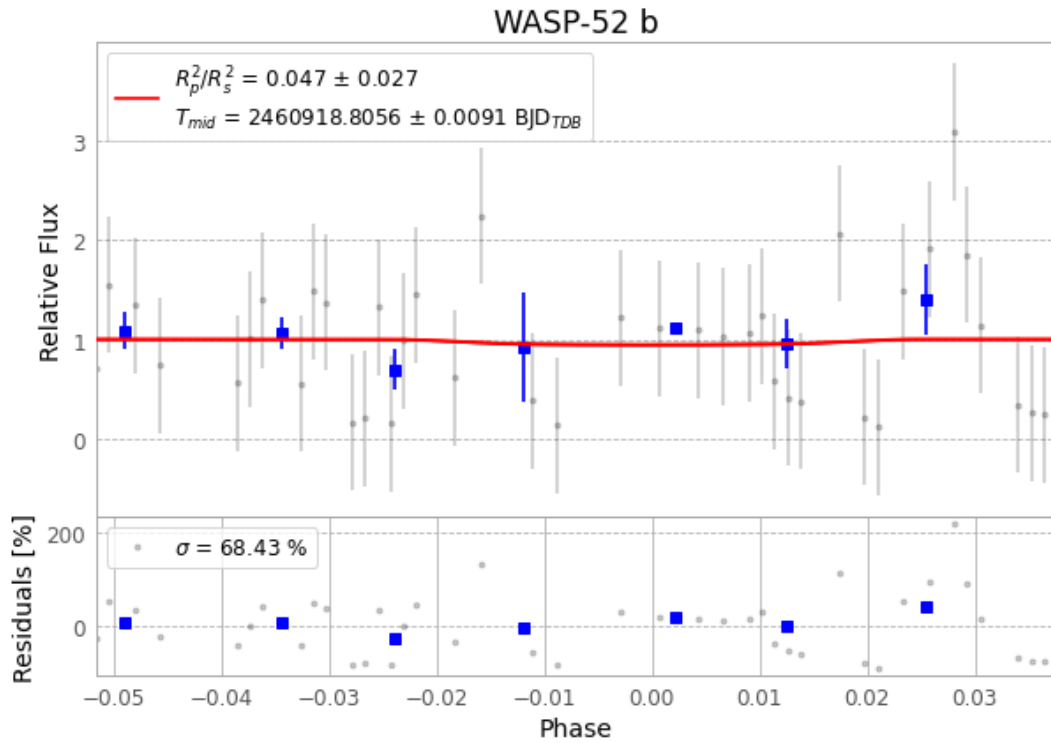
Figure 1 — FinalLightCurve_WASP-52 b_2025-08-30.png (SHA-256 fccac58659a8cde9...)
