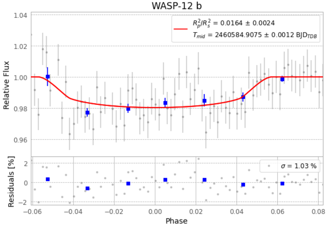
Figure 1 — FinalLightCurve_WASP-12 b_2024-10-01.png (SHA-256 b6cdb26163021d49...)
