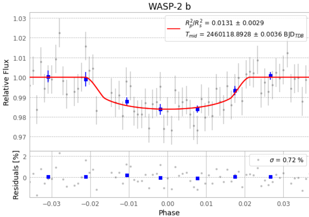
Figure 1 — FinalLightCurve_WASP-2 b_2023-06-23.png (SHA-256 38a91d76d492b0cf...)
