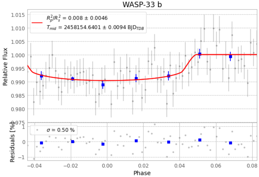
Figure 1 — FinalLightCurve_WASP-33 b_2018-02-04.png (SHA-256 f3d29cfd45042bc4...)
