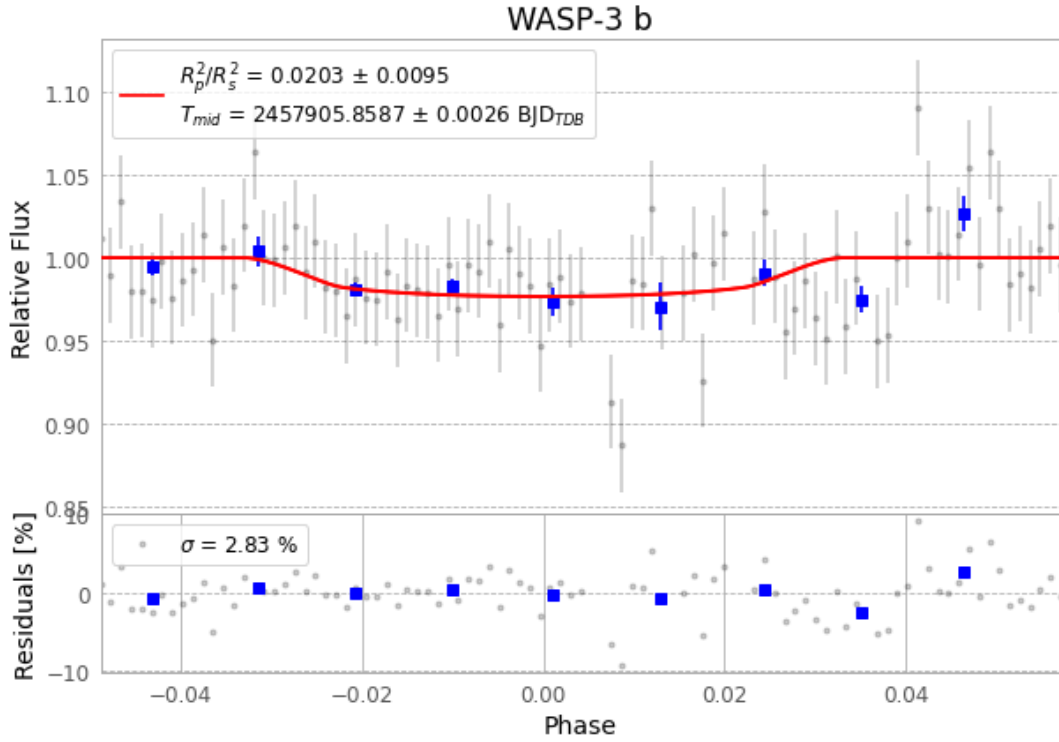
Figure 1 — FinalLightCurve_WASP-3 b_2017-05-31.png (SHA-256 782ff4e9d9ac1b91...)
