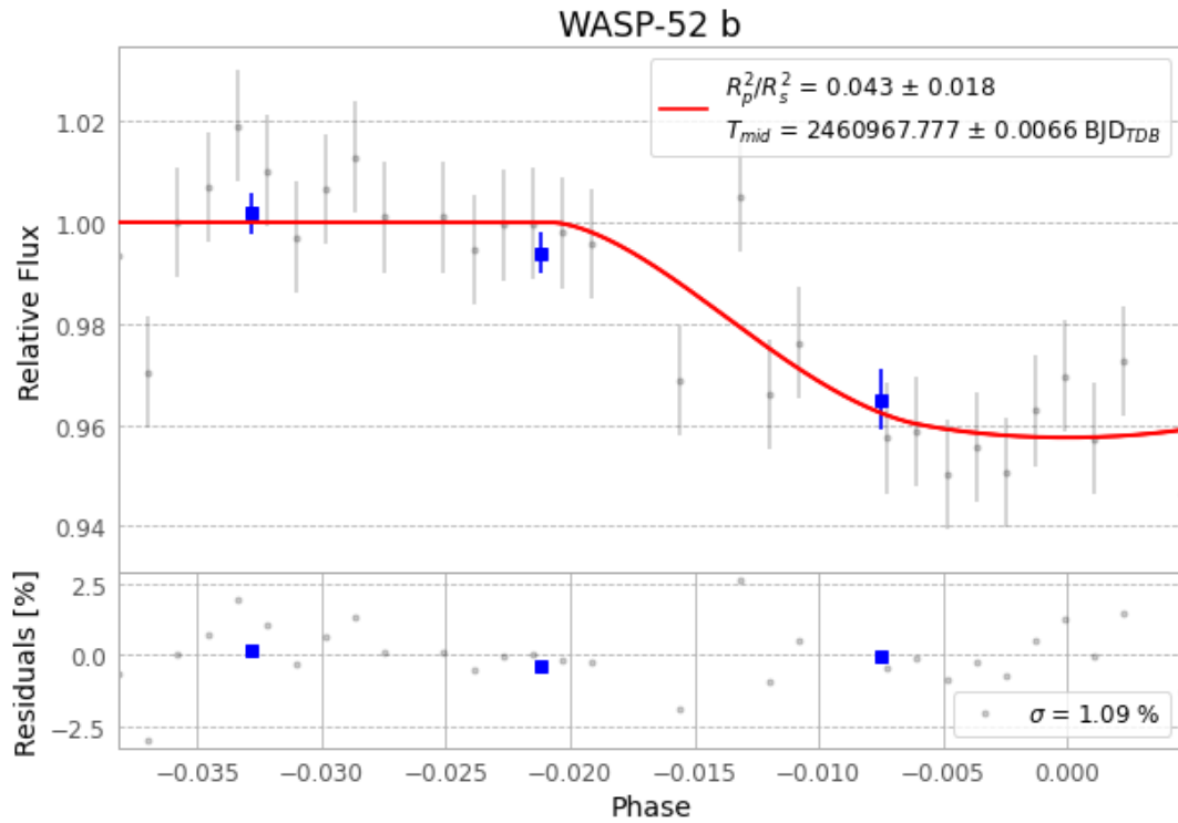
Figure 1 — FinalLightCurve_WASP-52 b_2025-10-18.png (SHA-256 fd6965cfca6e95b1...)
