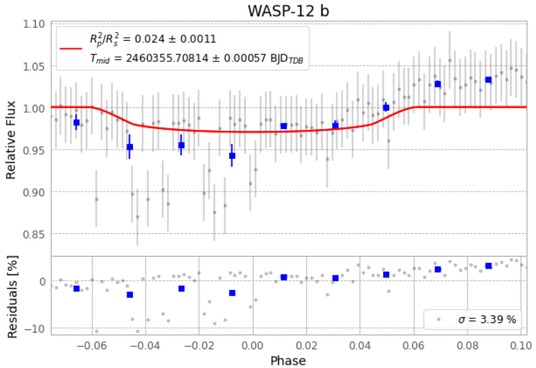
Figure 1 — FinalLightCurve_WASP-12 b_2024-02-14.png (SHA-256 04bd515612cecd2c...)
