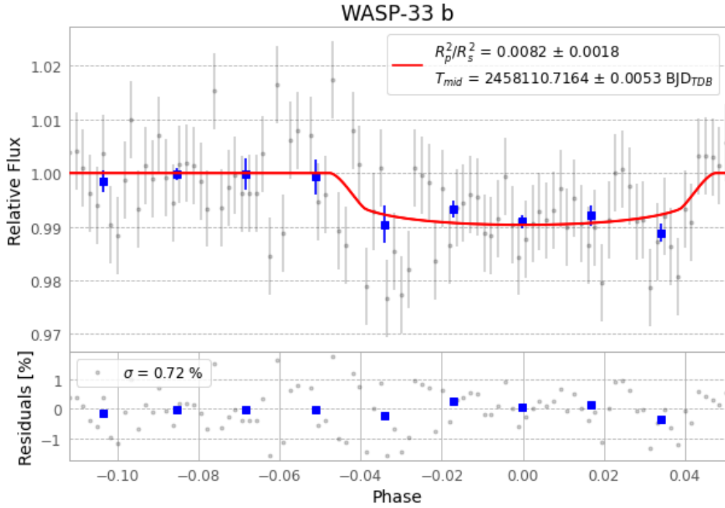
Figure 1 — FinalLightCurve_WASP-33 b_2017-12-22.png (SHA-256 f4be41c5b12eeeb6...)
