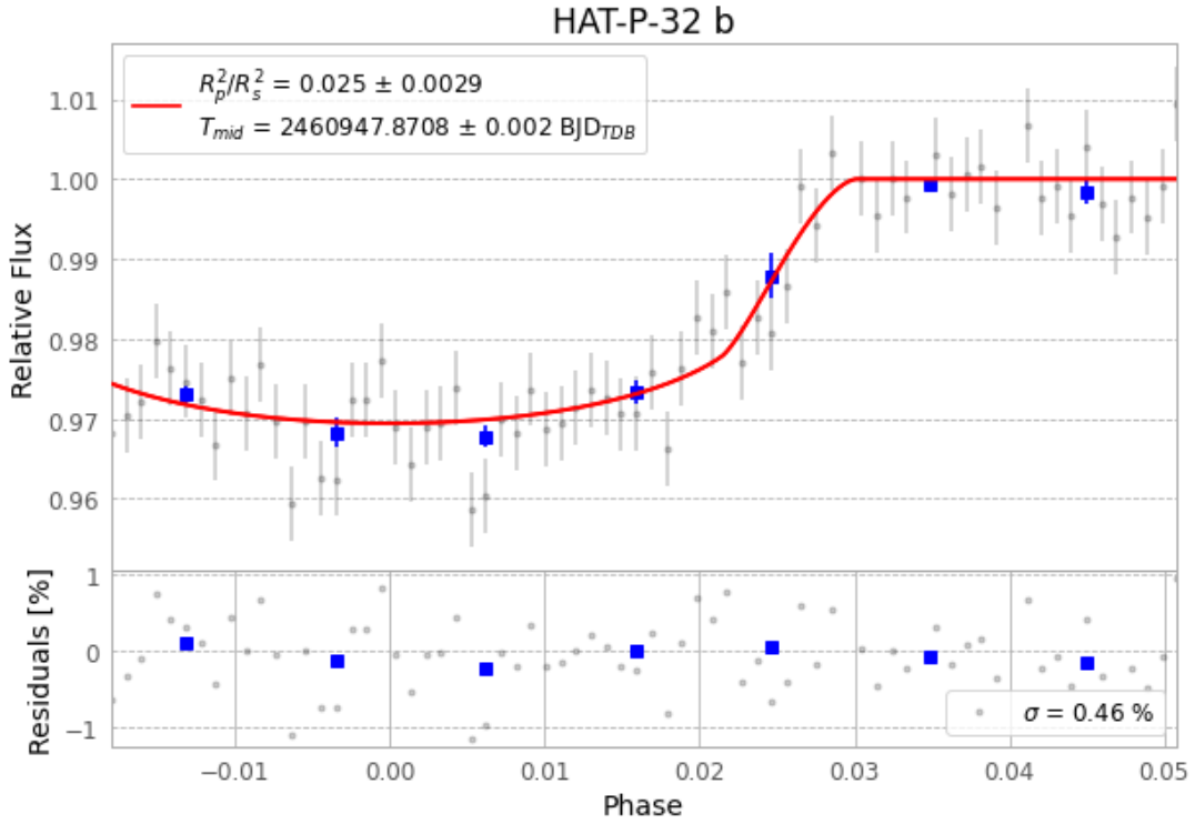
Figure 1 — FinalLightCurve_HAT-P-32 b_2025-09-29.png (SHA-256 9ac25fe43fd51dda...)
