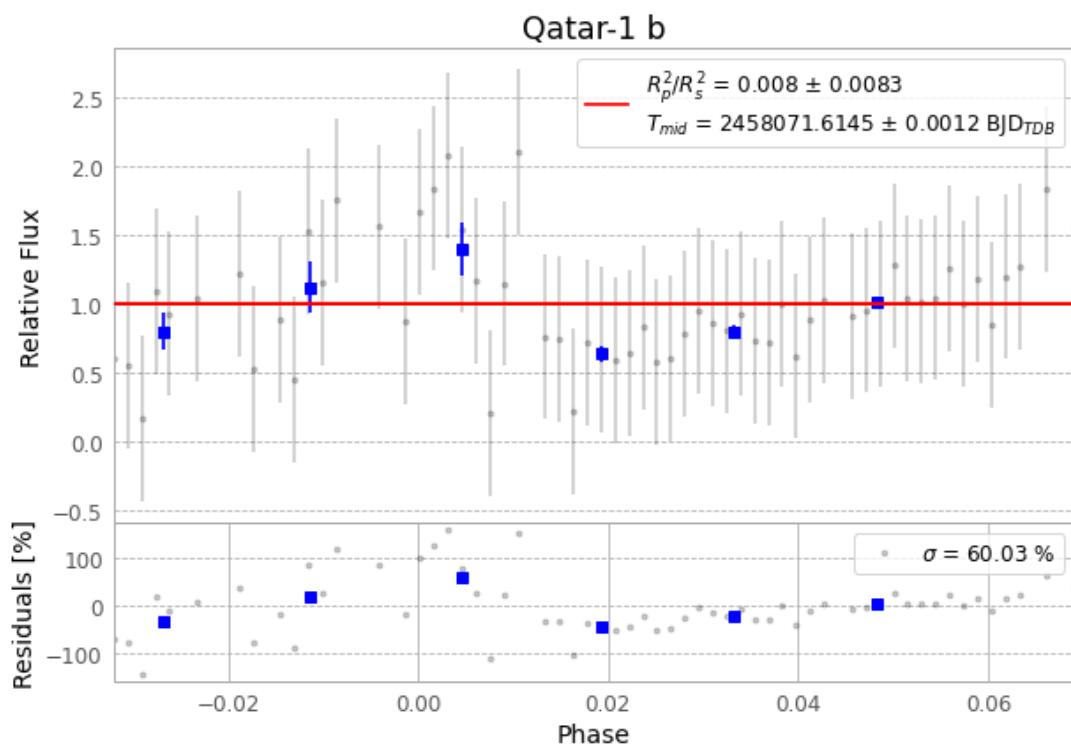
Figure 1 — FinalLightCurve_Qatar-1 b_2017-11-13.png (SHA-256 2a3c2b794f1ecab3...)
