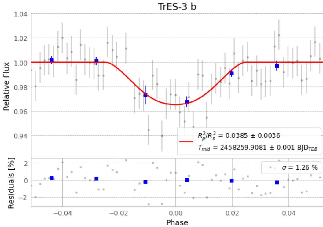
Figure 1 — FinalLightCurve_TrES-3 b_2018-05-21.png (SHA-256 2baa6a19a5aaa66d...)
