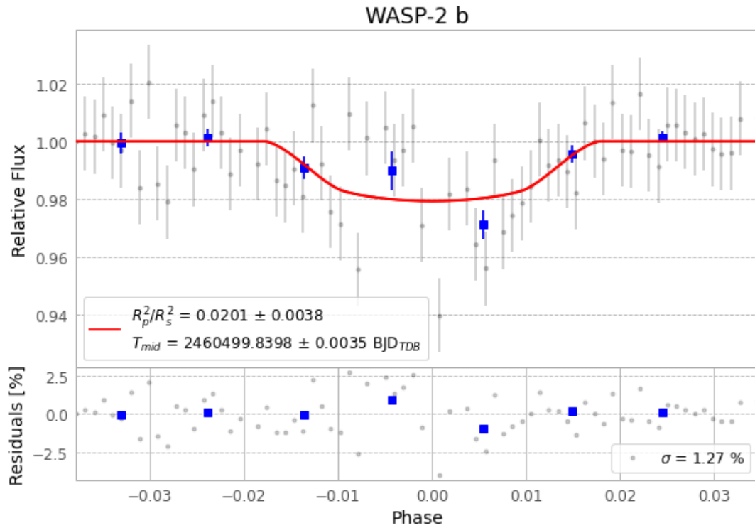
Figure 1 — FinalLightCurve_WASP-2 b_2024-07-07.png (SHA-256 c96f28167c23d2af...)
