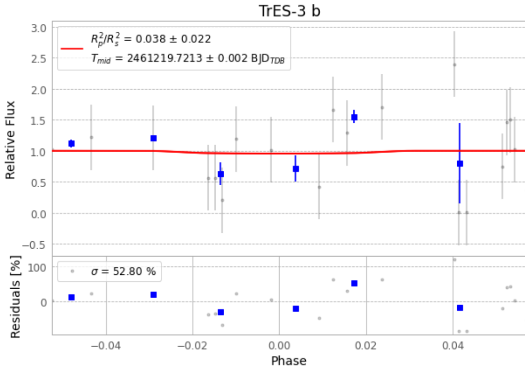
Figure 1 — FinalLightCurve_TrES-3 b_2026-06-27.png (SHA-256 11eac2dfc9f71e2f...)
