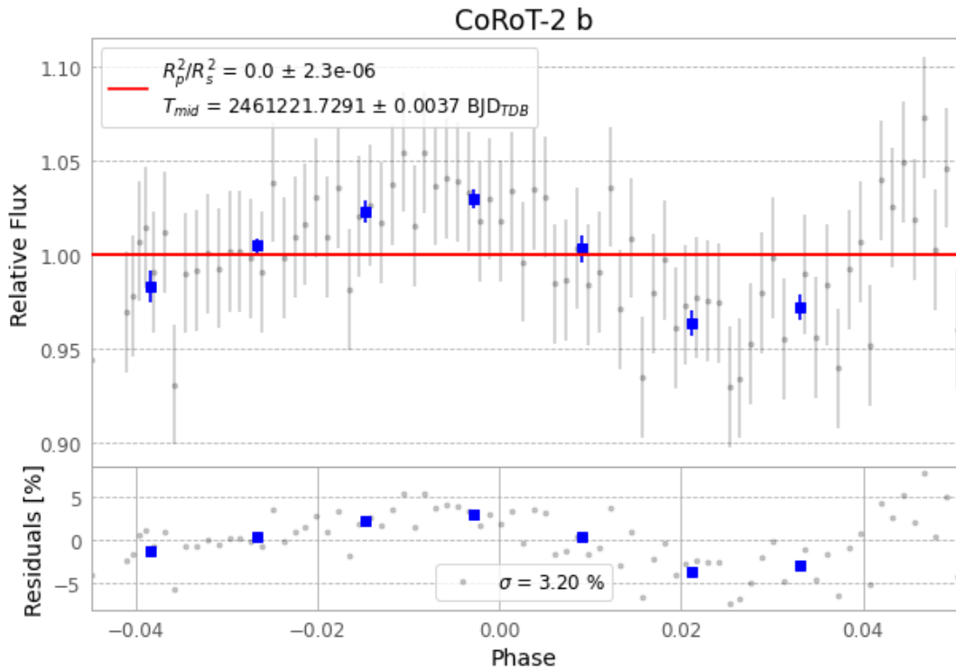
Figure 1 — FinalLightCurve_CoRoT-2 b_2026-06-29.png (SHA-256 0c41b58a20a8d985...)
