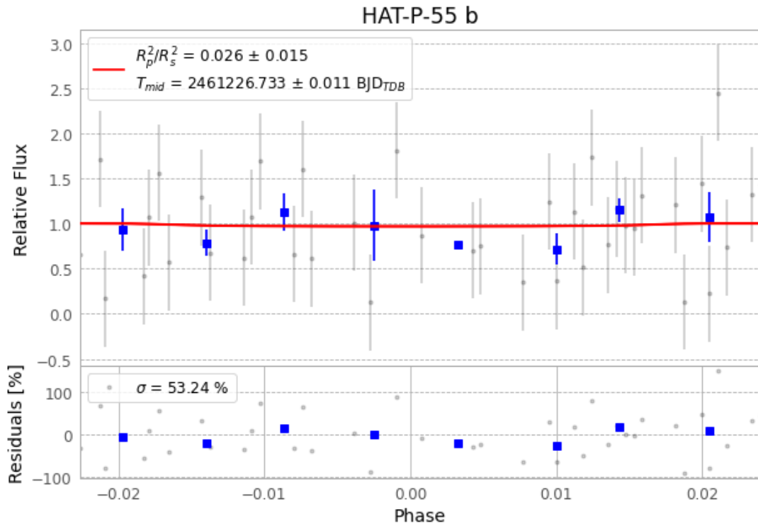
Figure 1 — FinalLightCurve_HAT-P-55 b_2026-07-04.png (SHA-256 5e44a232b211392b...)
