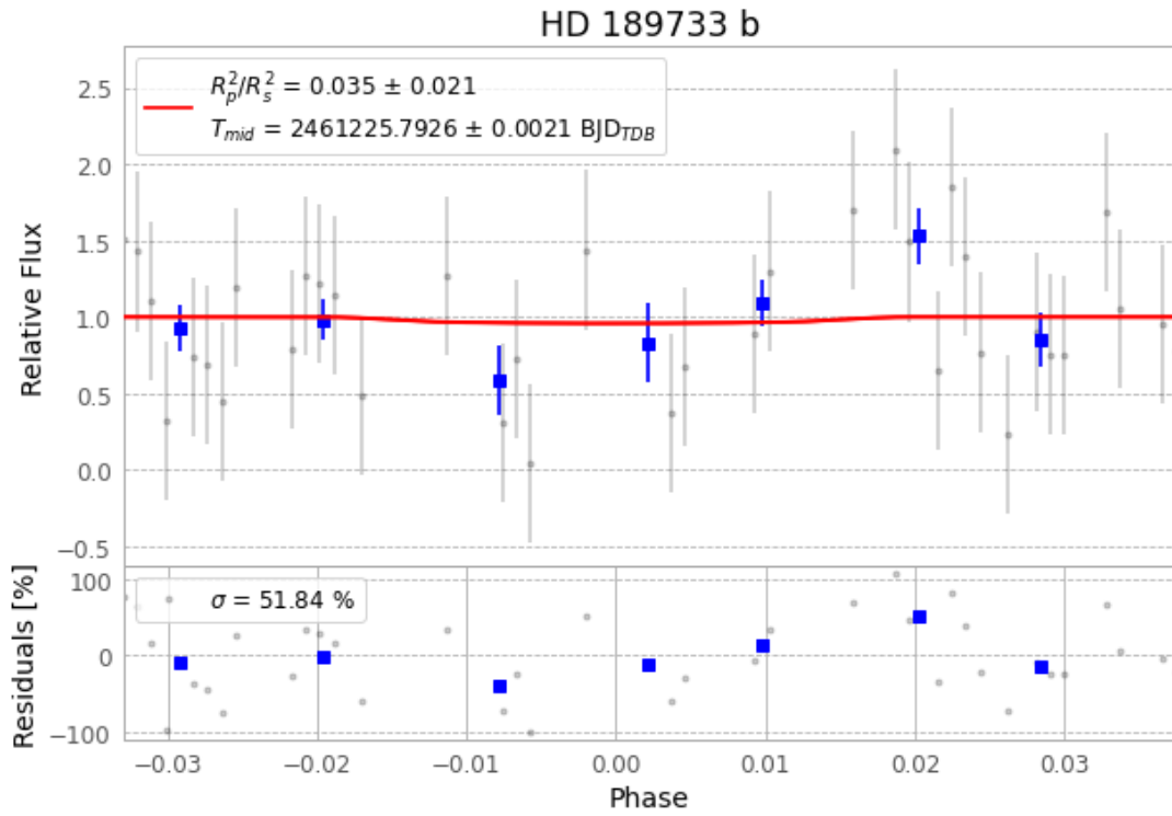
Figure 1 — FinalLightCurve_HD 189733 b_2026-07-04.png (SHA-256 8450a1f5cf6f9581...)
