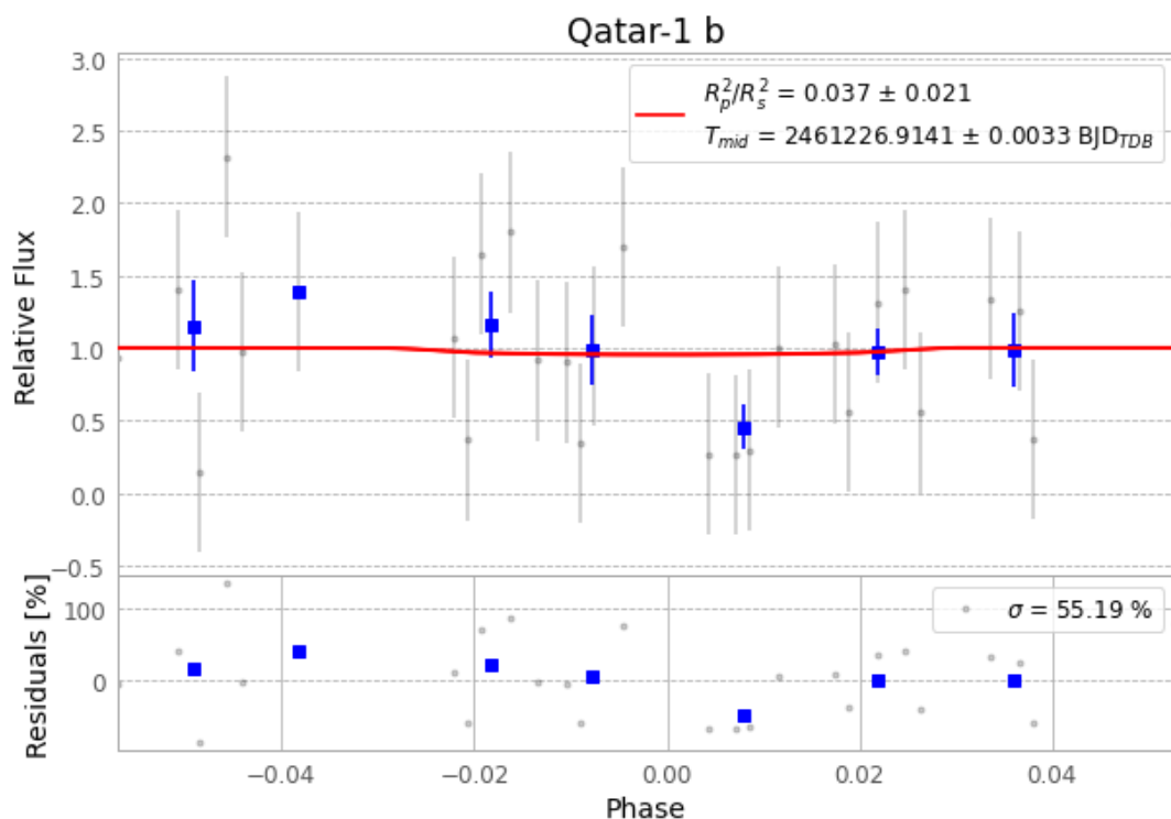
Figure 1 — FinalLightCurve_Qatar-1 b_2026-07-05.png (SHA-256 020320e6d66a32ea...)
