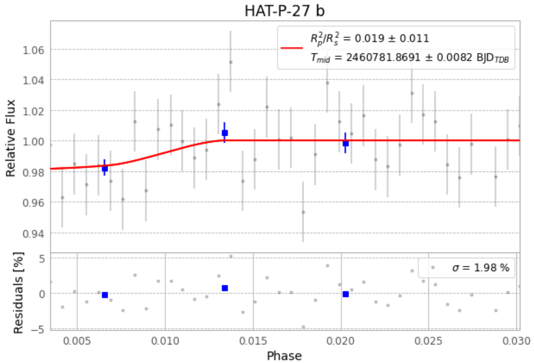
Figure 1 — FinalLightCurve_HAT-P-27 b_2025-04-16.png (SHA-256 fc625f2f6bcf08f6...)
