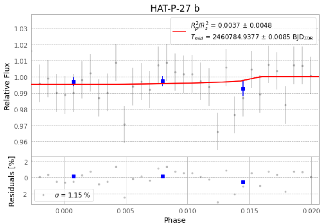
Figure 1 — FinalLightCurve_HAT-P-27 b_2025-04-19.png (SHA-256 ed59e2aa4bd23787...)
