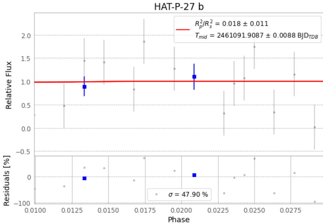
Figure 1 — FinalLightCurve_HAT-P-27 b_2026-02-20.png (SHA-256 b244d109090a53e6...)
