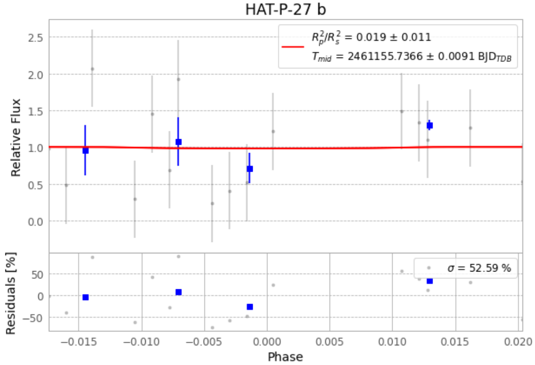
Figure 1 — FinalLightCurve_HAT-P-27 b_2026-04-24.png (SHA-256 8110cea1b30485ee...)
