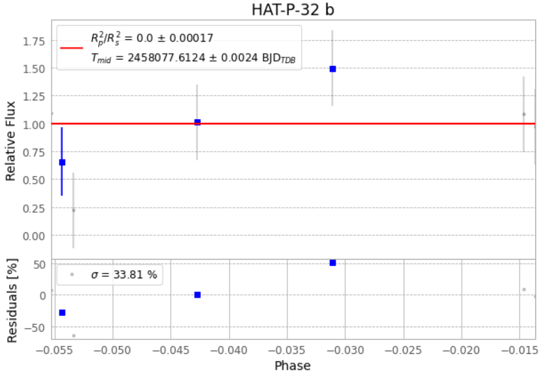
Figure 1 — FinalLightCurve_HAT-P-32 b_2017-11-21.png (SHA-256 f70360f6d59f685d...)
