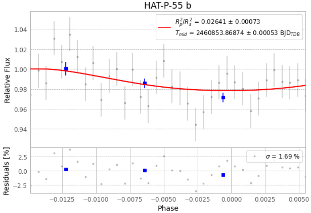
Figure 1 — FinalLightCurve_HAT-P-55 b_2025-06-27.png (SHA-256 7340f7c37b23e7da...)
