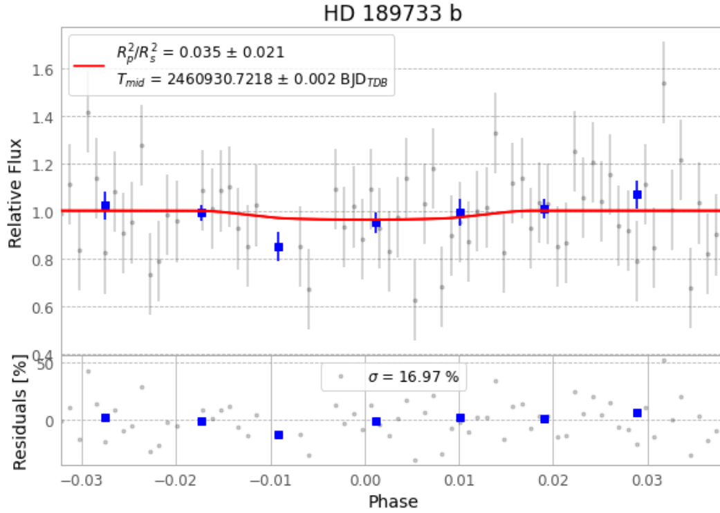
Figure 1 — FinalLightCurve_HD 189733 b_2025-09-11.png (SHA-256 a0432ecec3e91904...)
