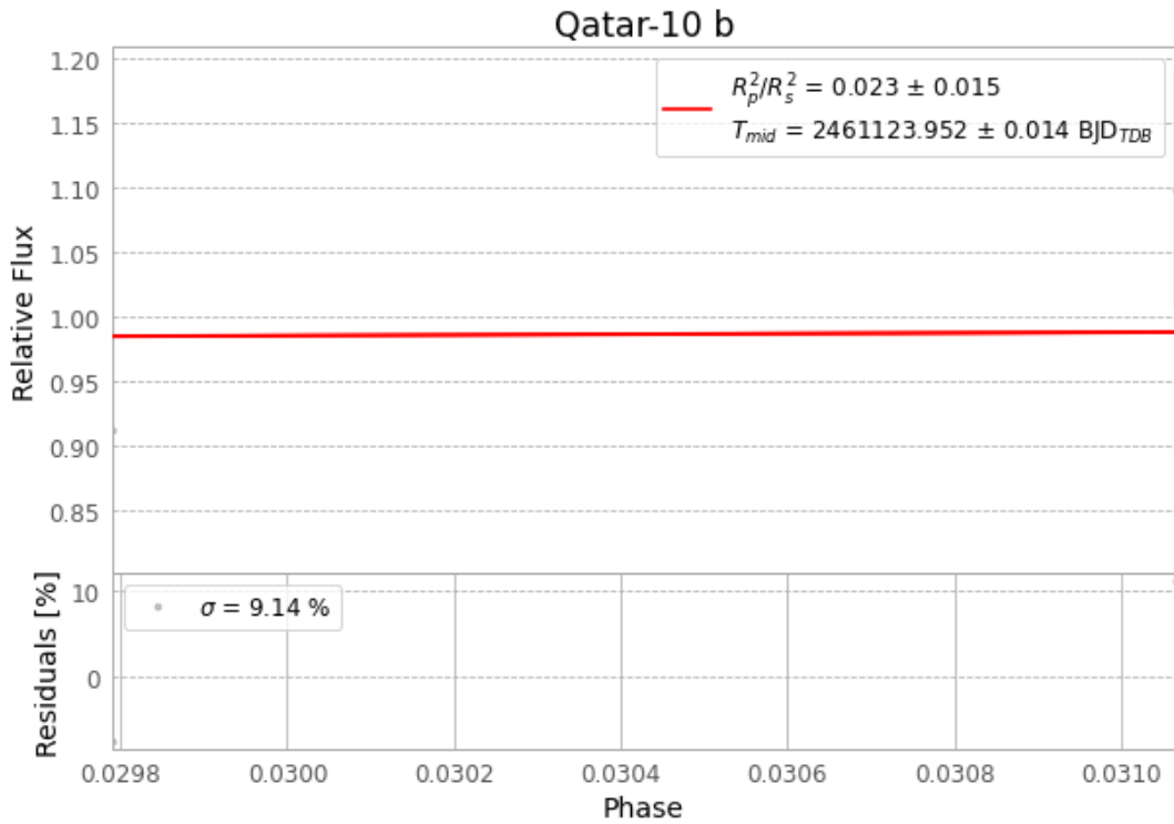
Figure 1 — FinalLightCurve_Qatar-10 b_2026-03-24.png (SHA-256 3fb0b03130df34ac...)
