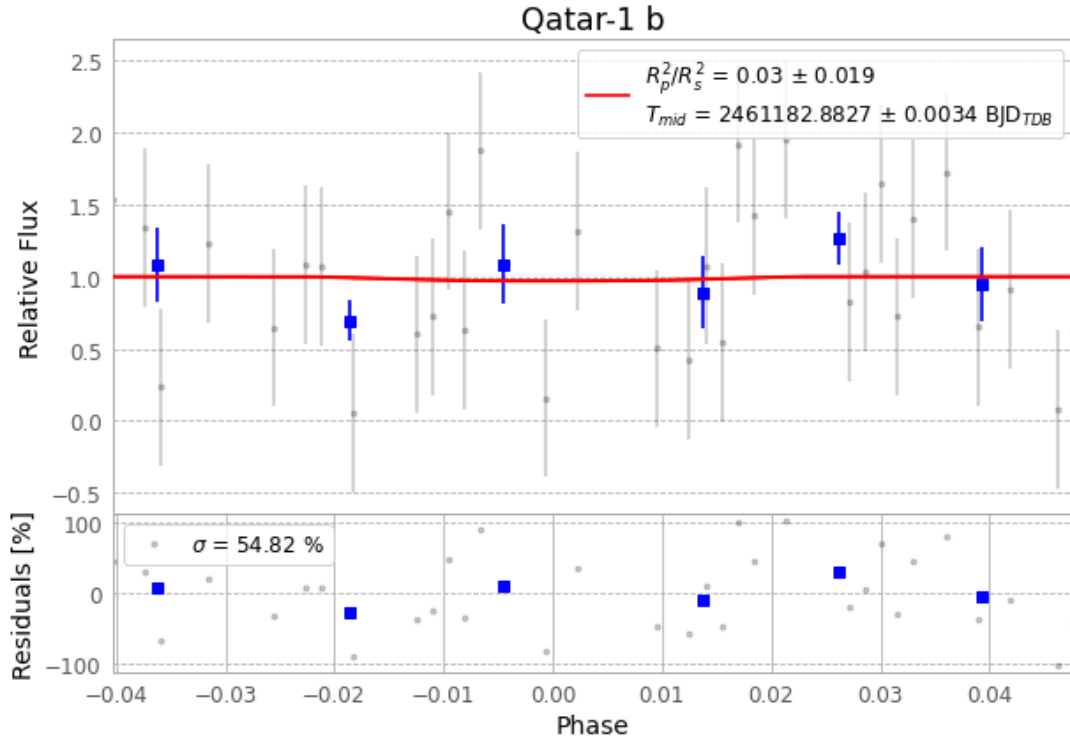
Figure 1 — FinalLightCurve_Qatar-1 b_2026-05-22.png (SHA-256 e7087401718a9d24...)
