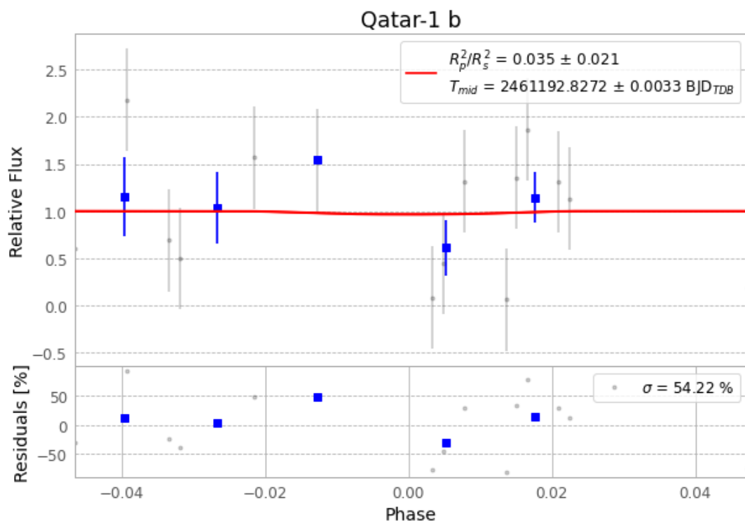
Figure 1 — FinalLightCurve_Qatar-1 b_2026-06-01.png (SHA-256 f3a3df938dd082e3...)
