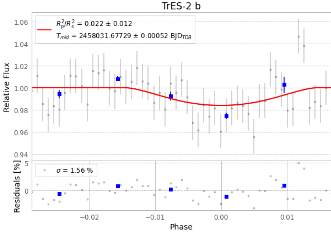
Figure 1 — FinalLightCurve_TrES-2 b_2017-10-04.png (SHA-256 908377a3e9745e7a...)
