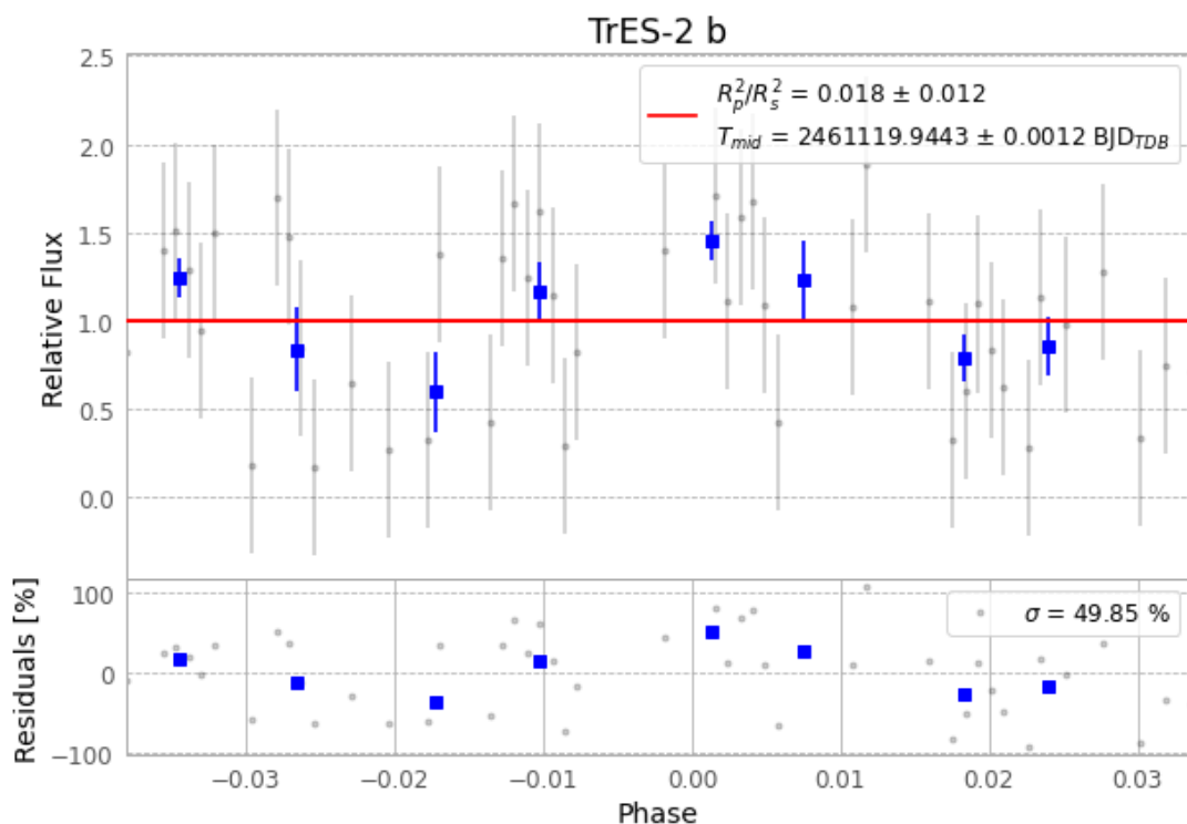
Figure 1 — FinalLightCurve_TrES-2 b_2026-03-20.png (SHA-256 386677bb57e3c57c...)
