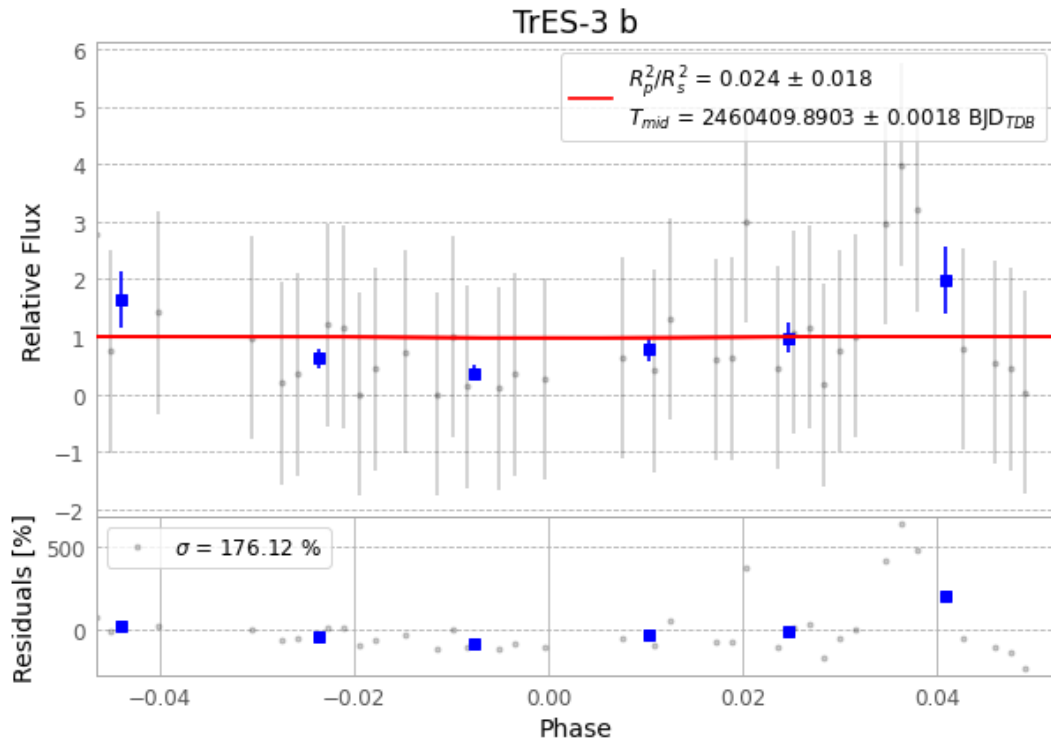
Figure 1 — FinalLightCurve_TrES-3 b_2024-04-09.png (SHA-256 ffc553170380a1b...)
